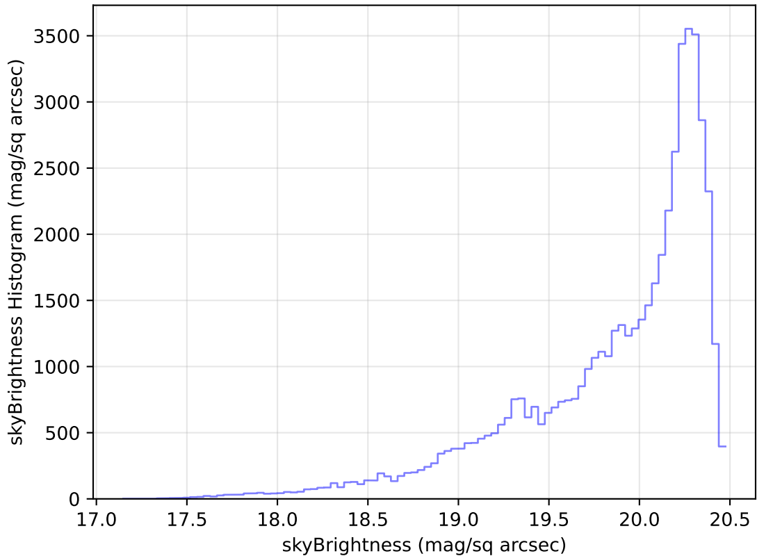
internal_u_expt45_nscale1.0v3.4_10yrs Yr 1 i band: skyBrightness Histogram
