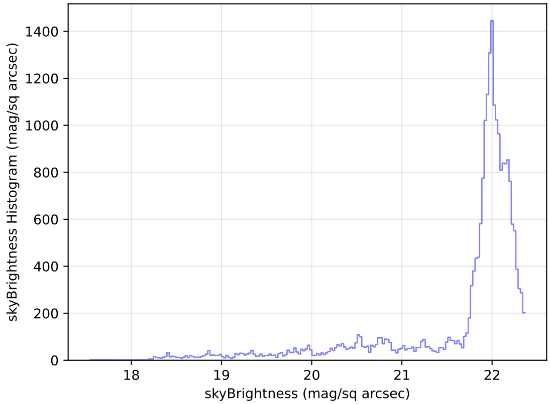
internal_u_expt45_nscale1.0v3.4_10yrs Yr 1 g band: skyBrightness Histogram
