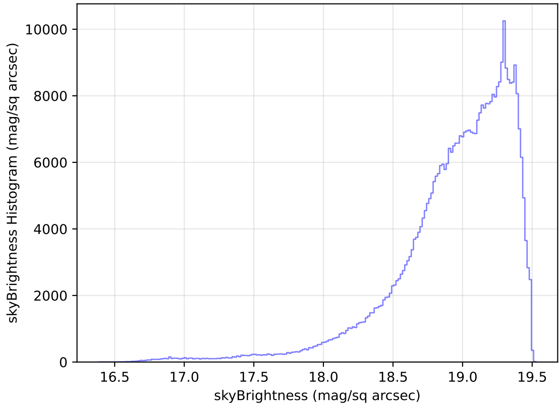
internal_u_expt45_nscale1.0v3.4_10yrs WFD z band: skyBrightness Histogram
