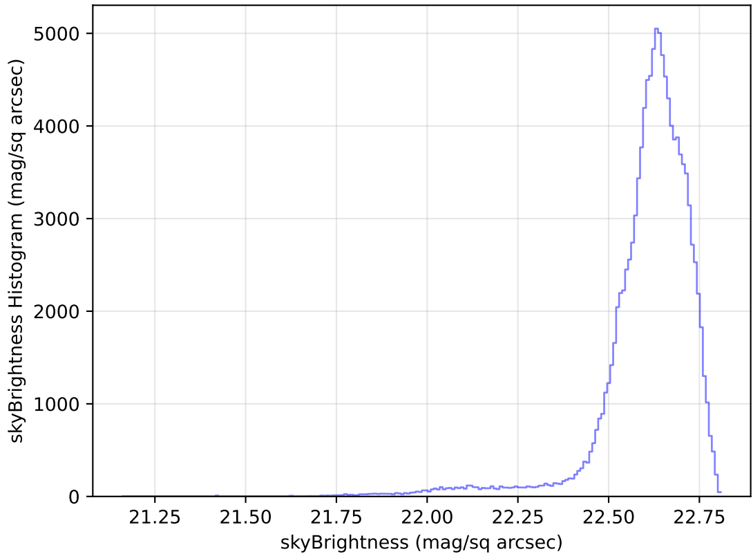
internal_u_expt45_nscale1.0v3.4_10yrs WFD u band: skyBrightness Histogram
