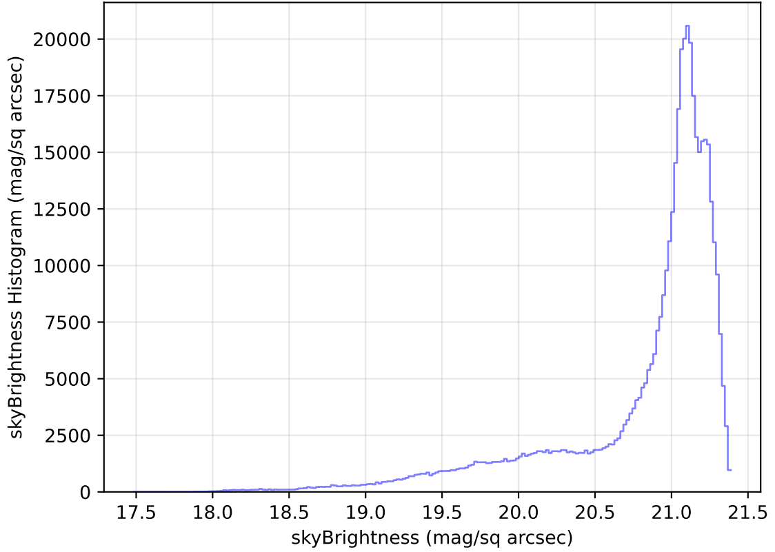
internal_u_expt45_nscale1.0v3.4_10yrs WFD r band: skyBrightness Histogram
