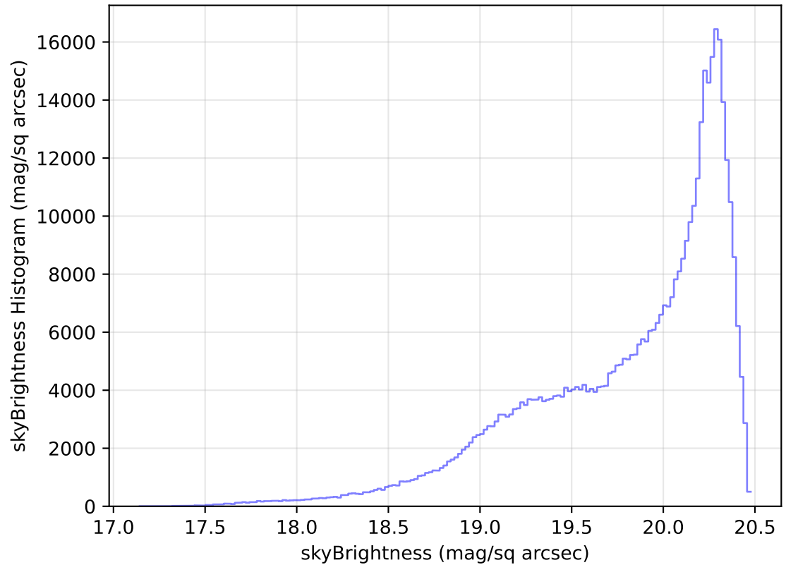
internal_u_expt45_nscale1.0v3.4_10yrs WFD i band: skyBrightness Histogram
