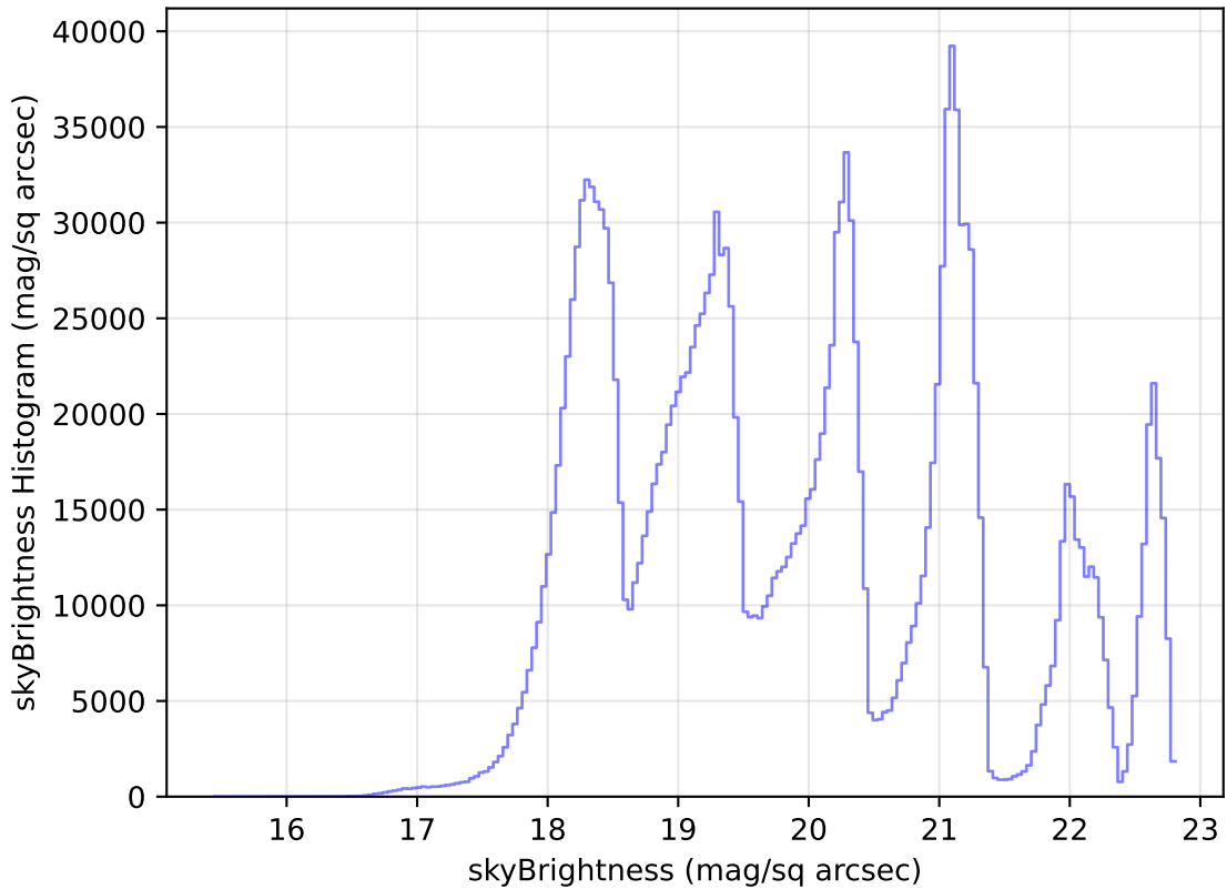
internal_u_expt45_nscale1.0v3.4_10yrs WFD all bands: skyBrightness Histogram
