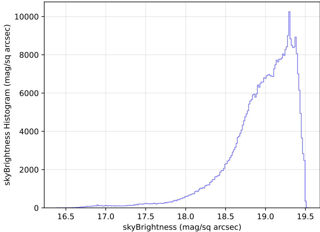
internal_u_expt45_nscale1.0v3.4_10yrs All sky z band: skyBrightness Histogram
