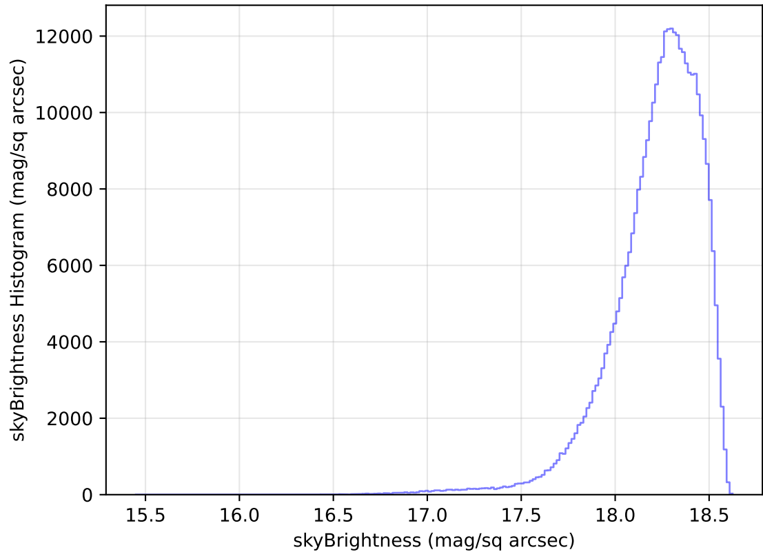
internal_u_expt45_nscale1.0v3.4_10yrs All sky y band: skyBrightness Histogram
