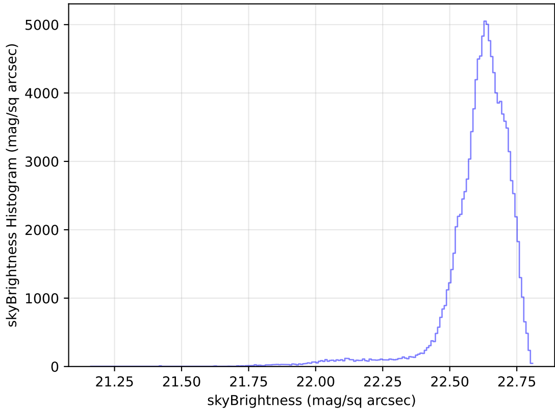
internal_u_expt45_nscale1.0v3.4_10yrs All sky u band: skyBrightness Histogram
