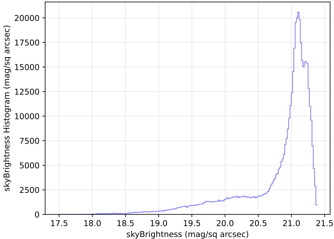
internal_u_expt45_nscale1.0v3.4_10yrs All sky r band: skyBrightness Histogram
