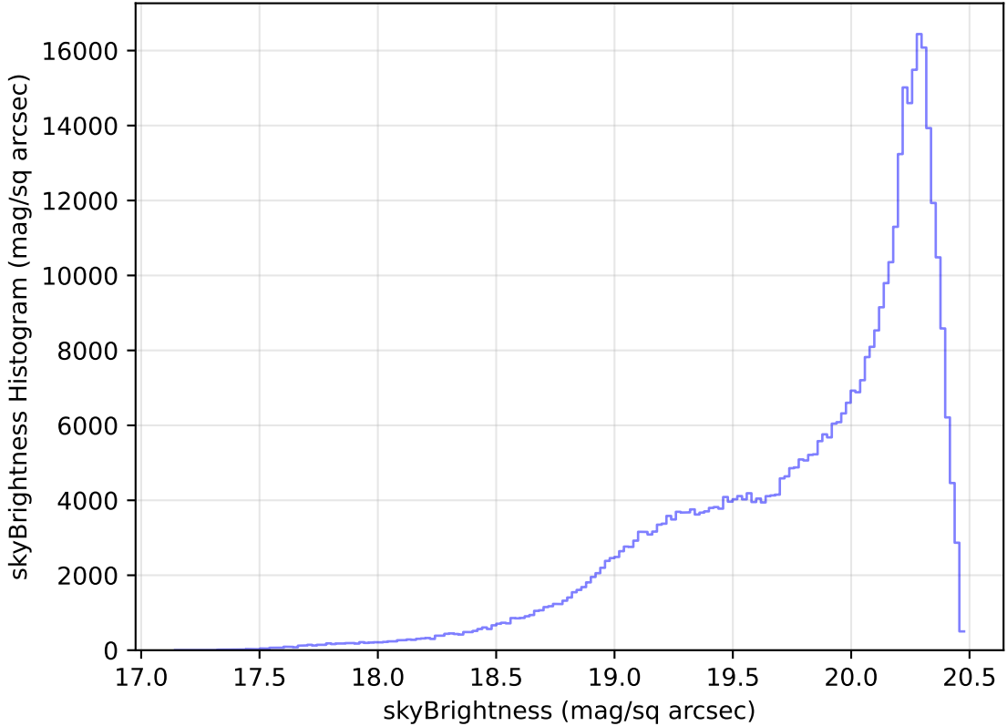
internal_u_expt45_nscale1.0v3.4_10yrs All sky i band: skyBrightness Histogram
