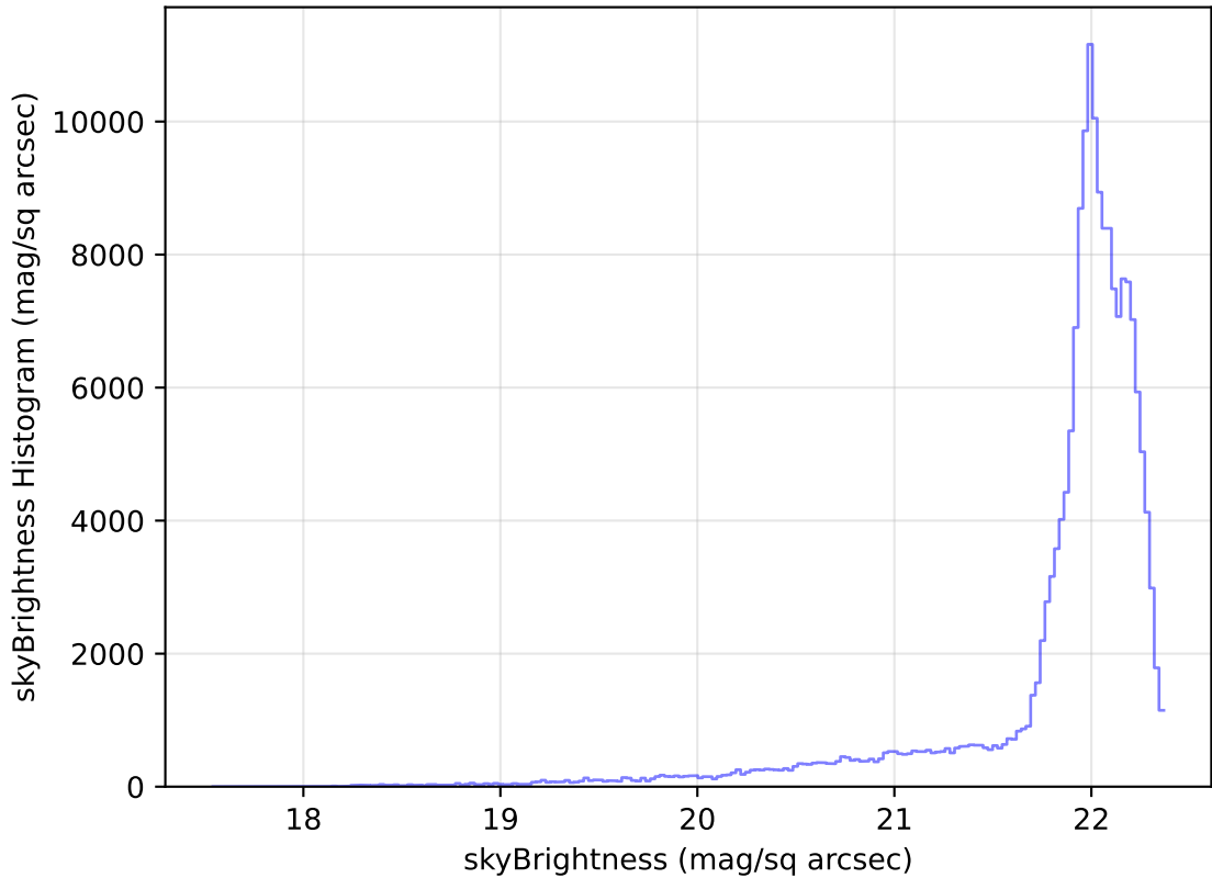
internal_u_expt45_nscale1.0v3.4_10yrs All sky g band: skyBrightness Histogram
