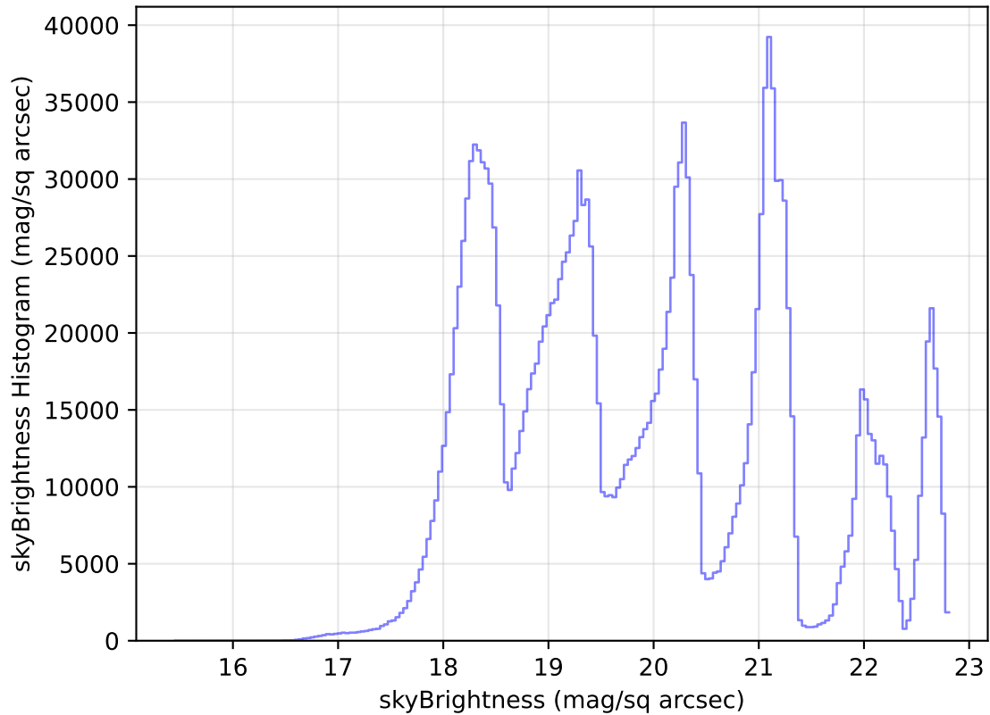
internal_u_expt45_nscale1.0v3.4_10yrs All sky all bands: skyBrightness Histogram
