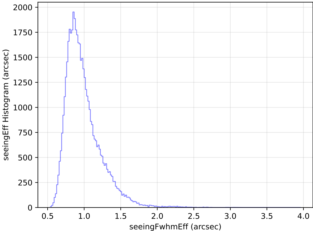
internal_u_expt45_nscale1.0v3.4_10yrs Yr 1 y band: seeingEff Histogram
