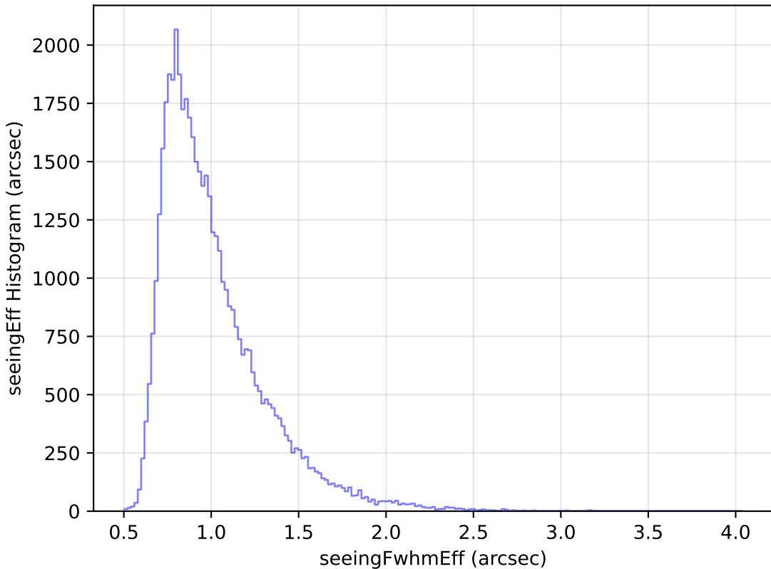
internal_u_expt45_nscale1.0v3.4_10yrs Yr 1 r band: seeingEff Histogram
