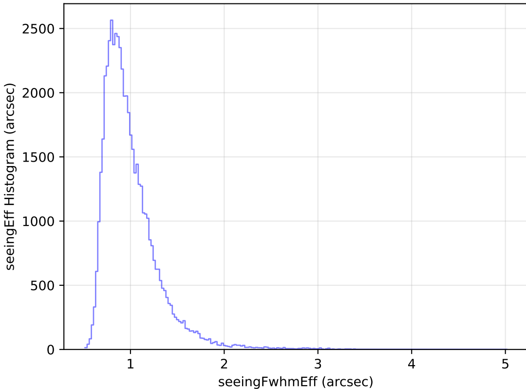
internal_u_expt45_nscale1.0v3.4_10yrs Yr 1 i band: seeingEff Histogram
