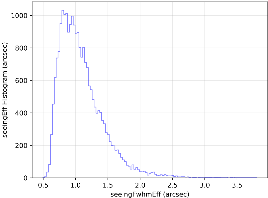
internal_u_expt45_nscale1.0v3.4_10yrs Yr 1 g band: seeingEff Histogram
