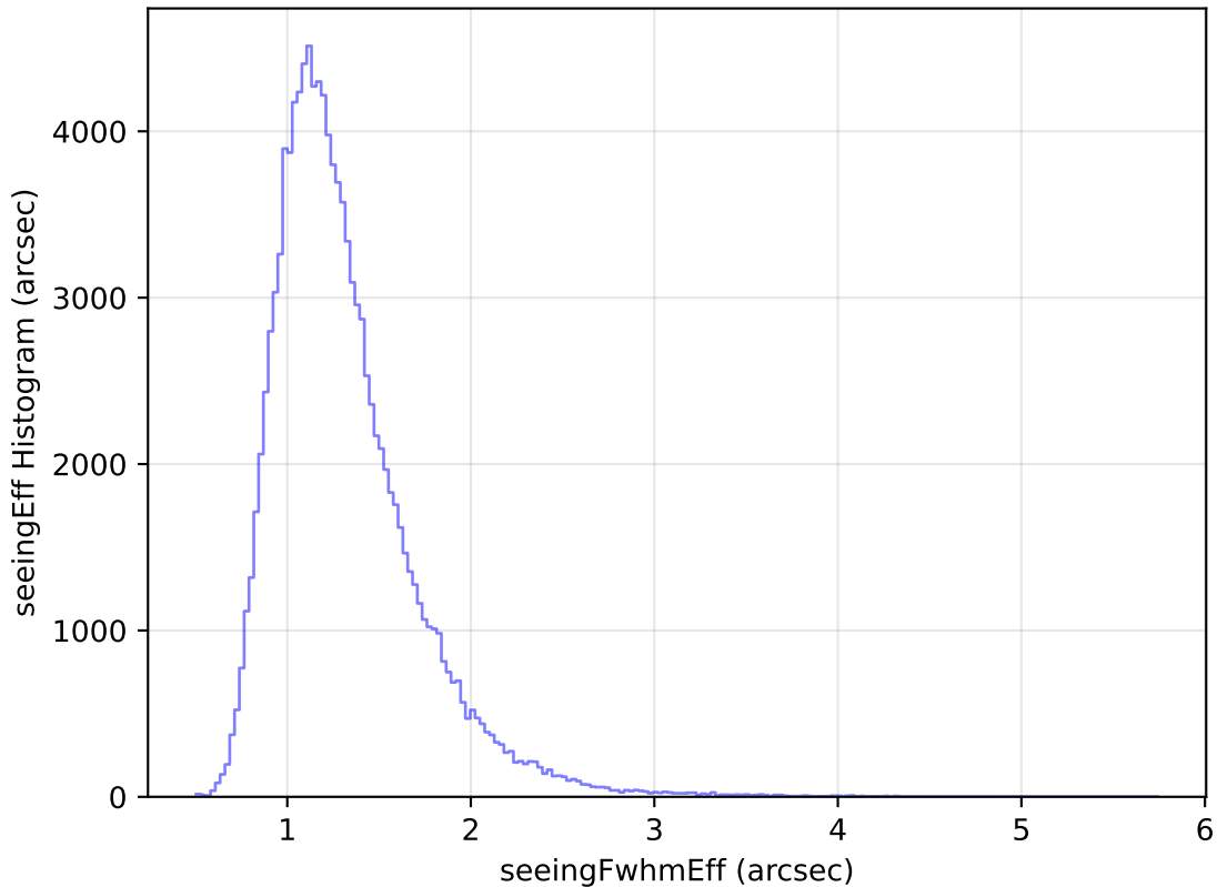
internal_u_expt45_nscale1.0v3.4_10yrs WFD u band: seeingEff Histogram
