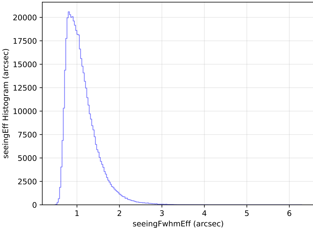
internal_u_expt45_nscale1.0v3.4_10yrs WFD r band: seeingEff Histogram
