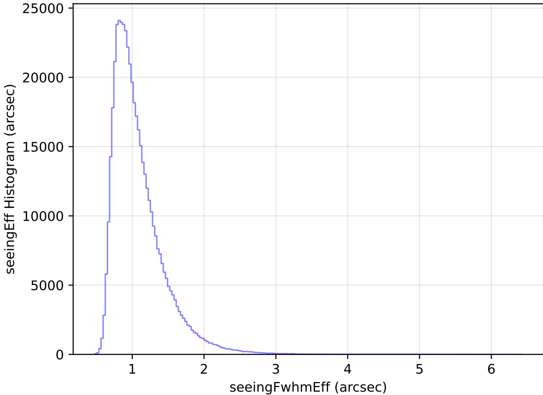
internal_u_expt45_nscale1.0v3.4_10yrs WFD i band: seeingEff Histogram
