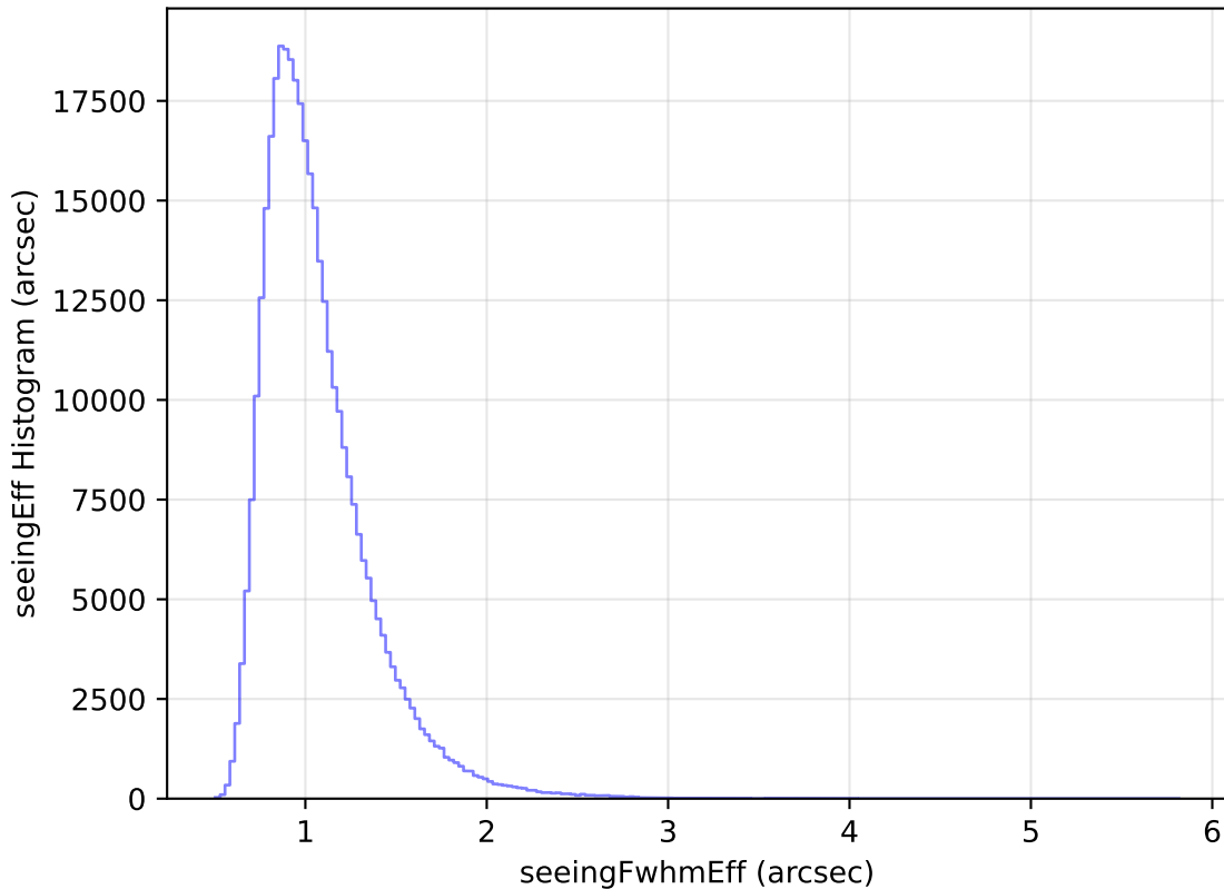
internal_u_expt45_nscale1.0v3.4_10yrs All sky y band: seeingEff Histogram
