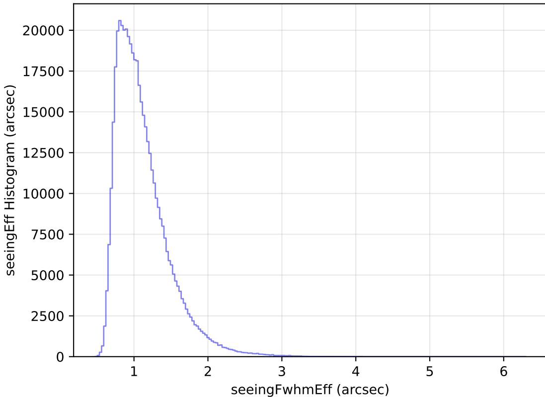
internal_u_expt45_nscale1.0v3.4_10yrs All sky r band: seeingEff Histogram
