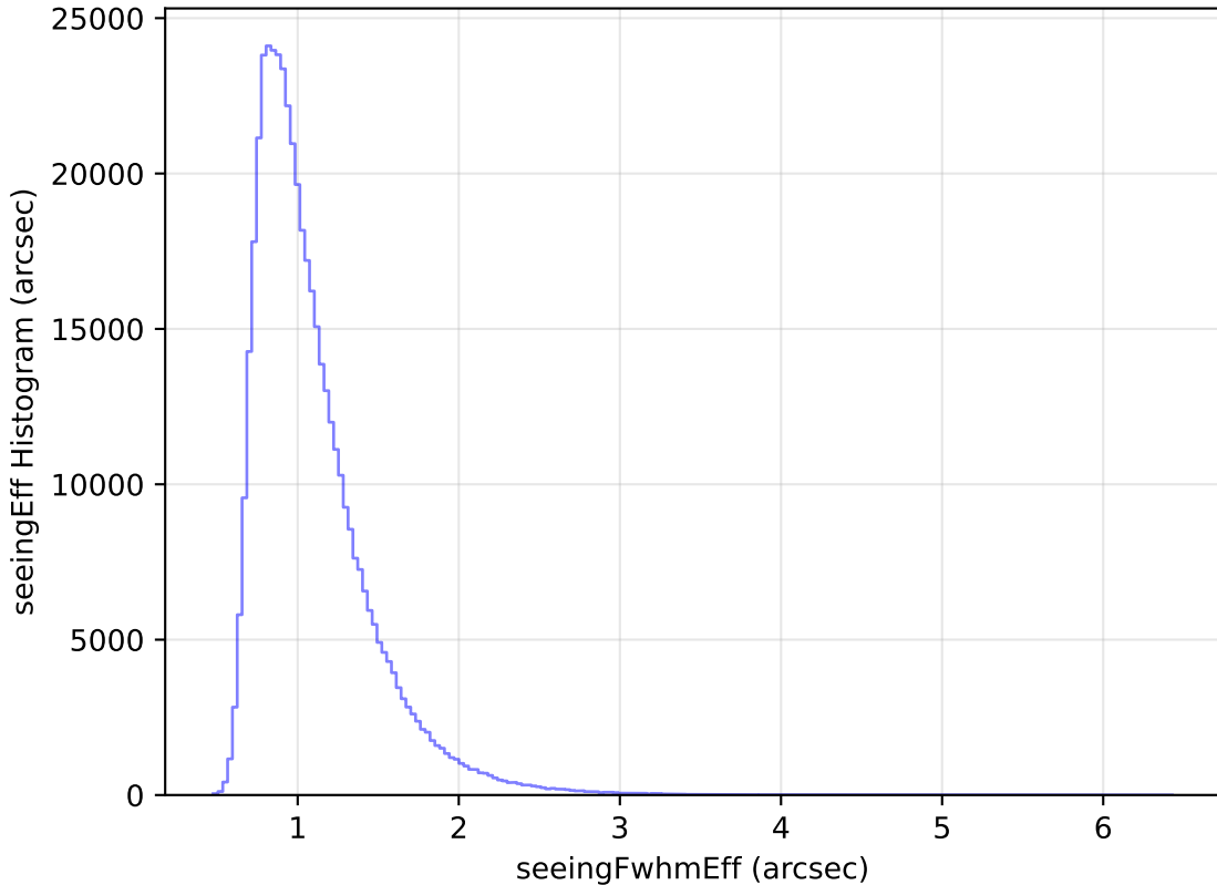
internal_u_expt45_nscale1.0v3.4_10yrs All sky i band: seeingEff Histogram
