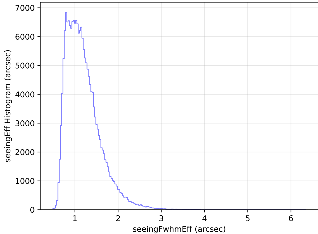
internal_u_expt45_nscale1.0v3.4_10yrs All sky g band: seeingEff Histogram
