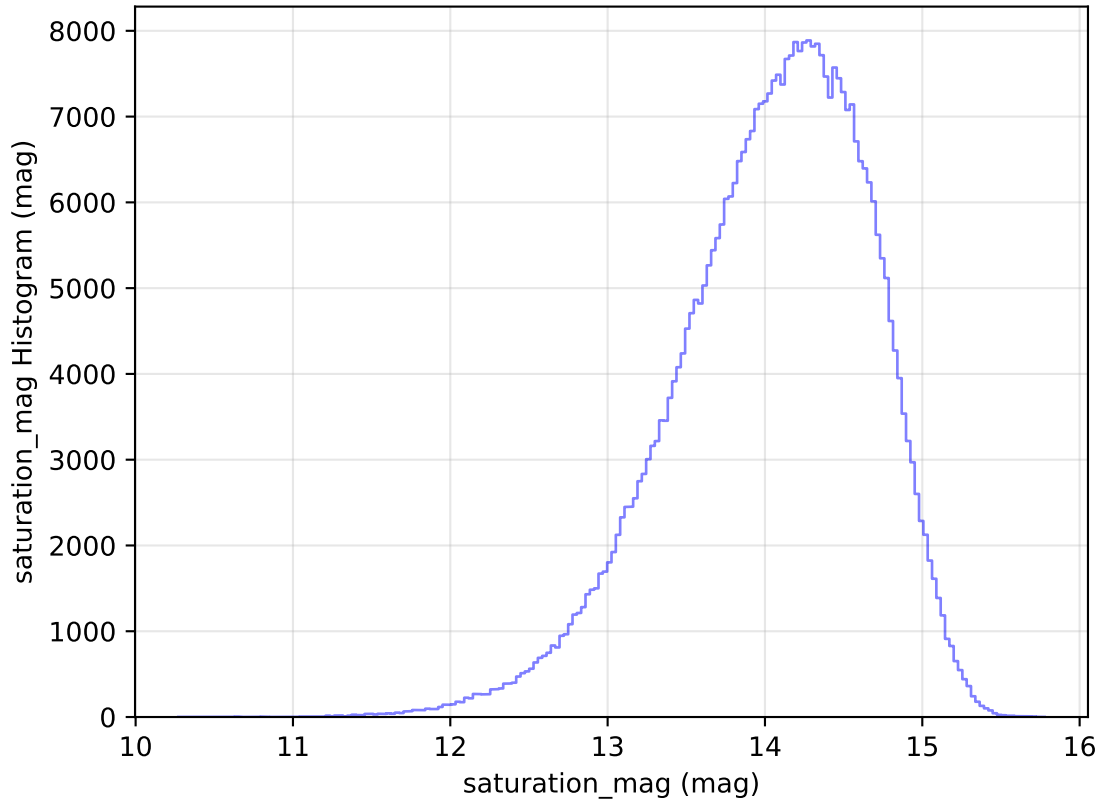
internal_u_expt45_nscale1.0v3.4_10yrs WFD z band: saturation_mag Histogram
