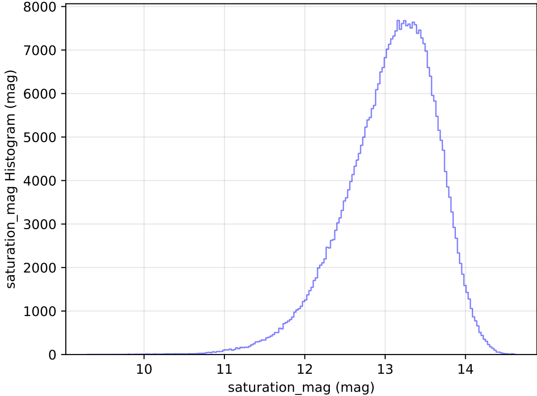
internal_u_expt45_nscale1.0v3.4_10yrs WFD y band: saturation_mag Histogram
