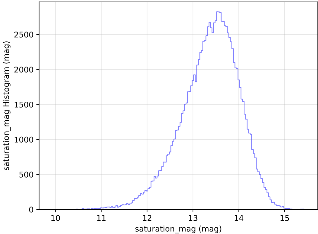
internal_u_expt45_nscale1.0v3.4_10yrs WFD u band: saturation_mag Histogram
