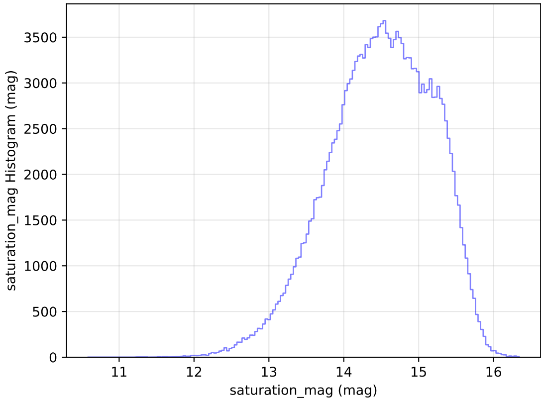
internal_u_expt45_nscale1.0v3.4_10yrs WFD g band: saturation_mag Histogram
