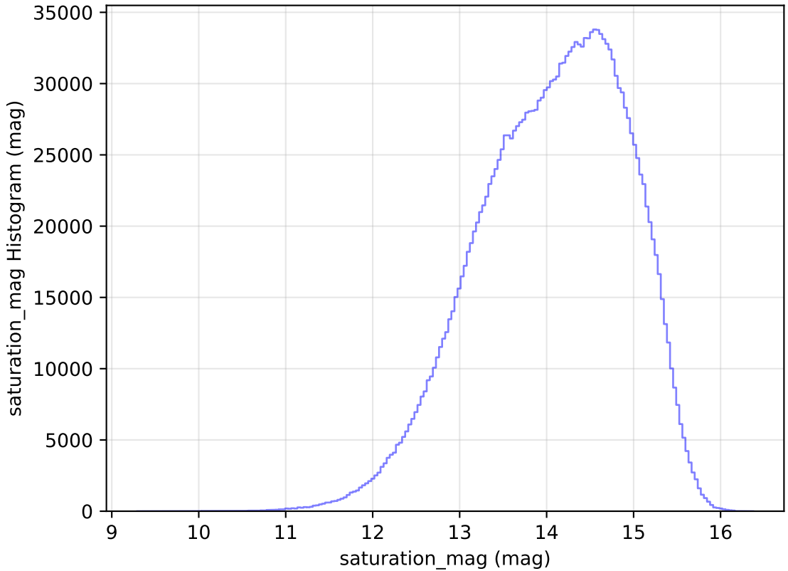
internal_u_expt45_nscale1.0v3.4_10yrs WFD all bands: saturation_mag Histogram
