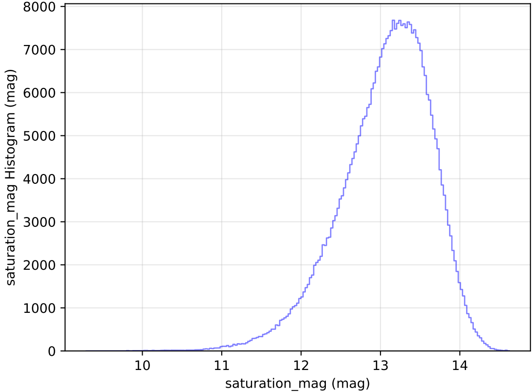
internal_u_expt45_nscale1.0v3.4_10yrs All sky y band: saturation_mag Histogram
