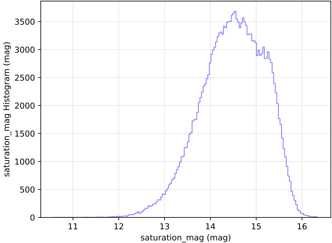
internal_u_expt45_nscale1.0v3.4_10yrs All sky g band: saturation_mag Histogram
