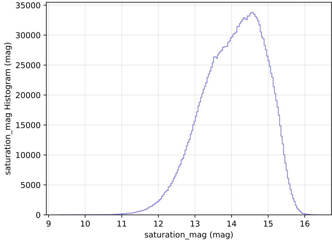
internal_u_expt45_nscale1.0v3.4_10yrs All sky all bands: saturation_mag Histogram
