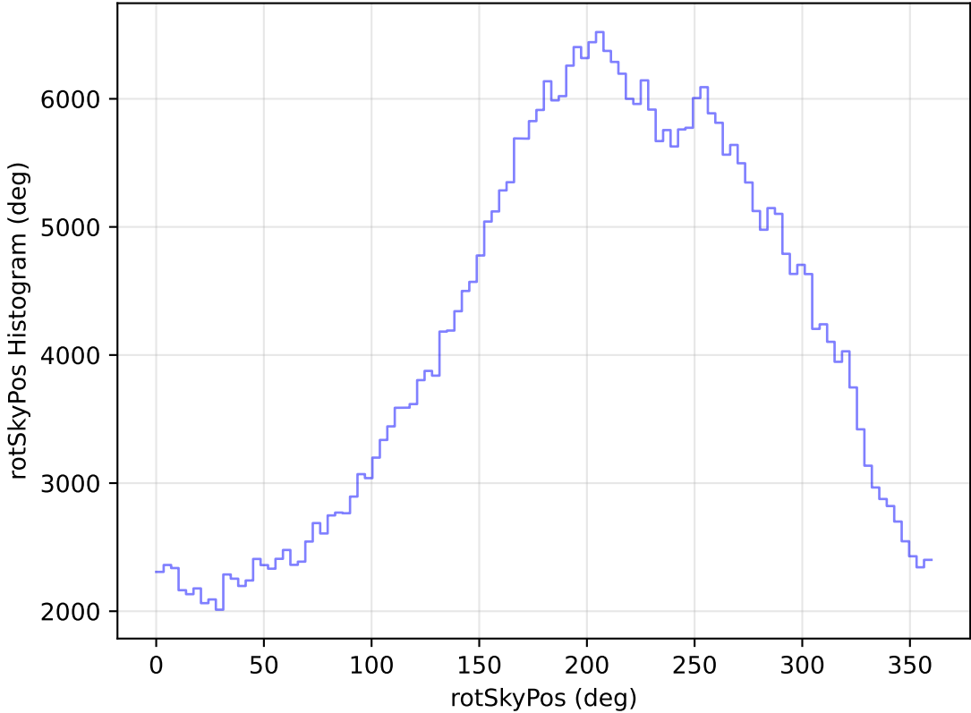
internal_u_expt45_nscale1.0v3.4_10yrs WFD z band: rotSkyPos Histogram
