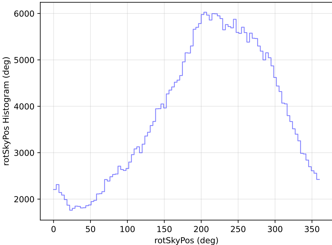
internal_u_expt45_nscale1.0v3.4_10yrs WFD y band: rotSkyPos Histogram
