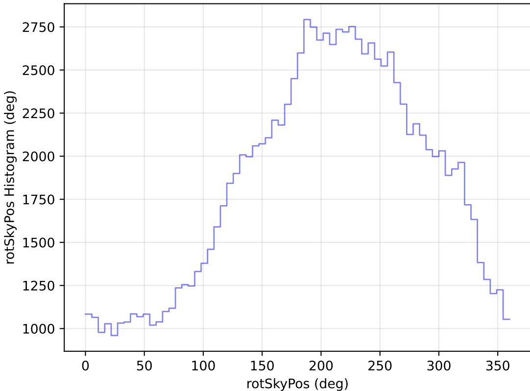
internal_u_expt45_nscale1.0v3.4_10yrs WFD u band: rotSkyPos Histogram
