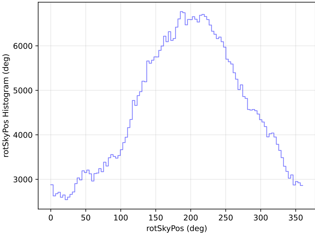
internal_u_expt45_nscale1.0v3.4_10yrs WFD r band: rotSkyPos Histogram
