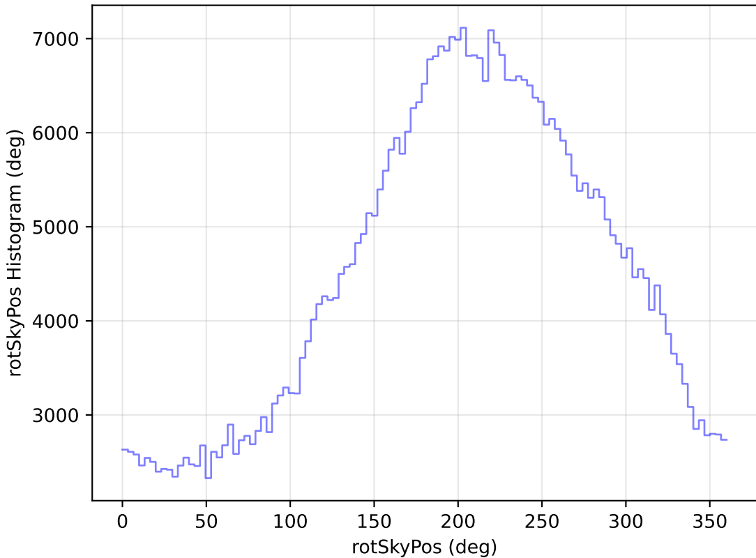
internal_u_expt45_nscale1.0v3.4_10yrs WFD i band: rotSkyPos Histogram
