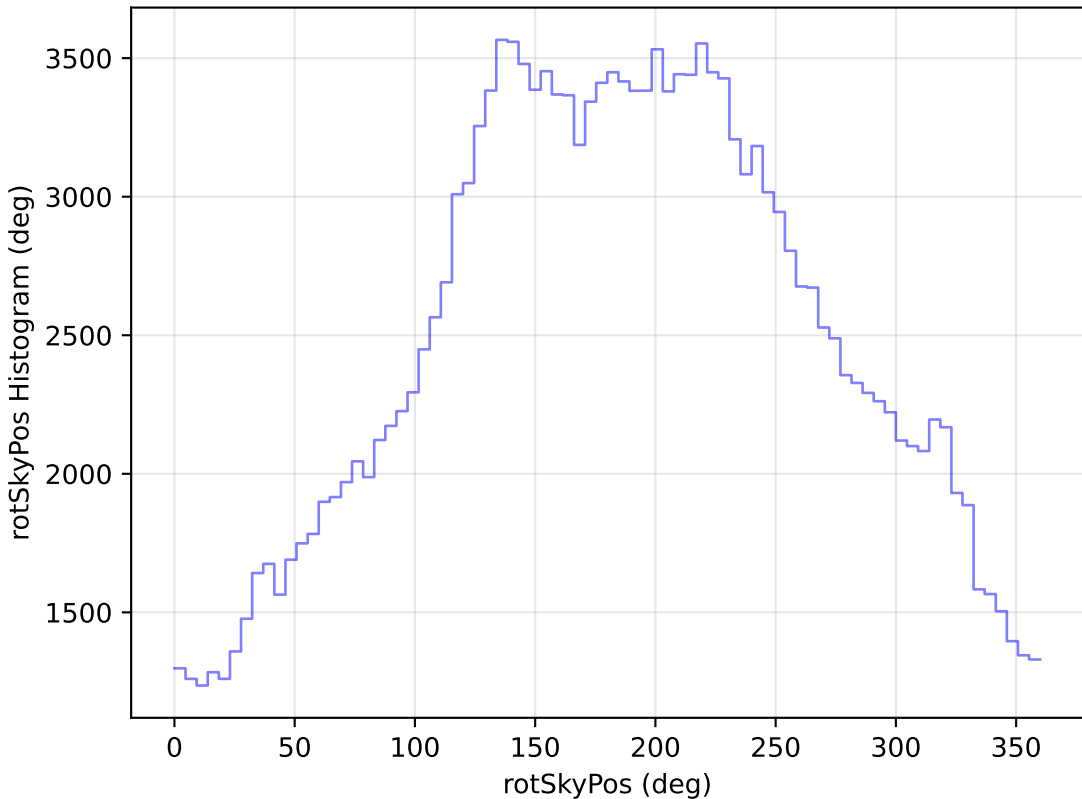
internal_u_expt45_nscale1.0v3.4_10yrs WFD g band: rotSkyPos Histogram
