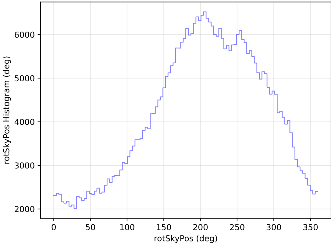
internal_u_expt45_nscale1.0v3.4_10yrs All sky z band: rotSkyPos Histogram
