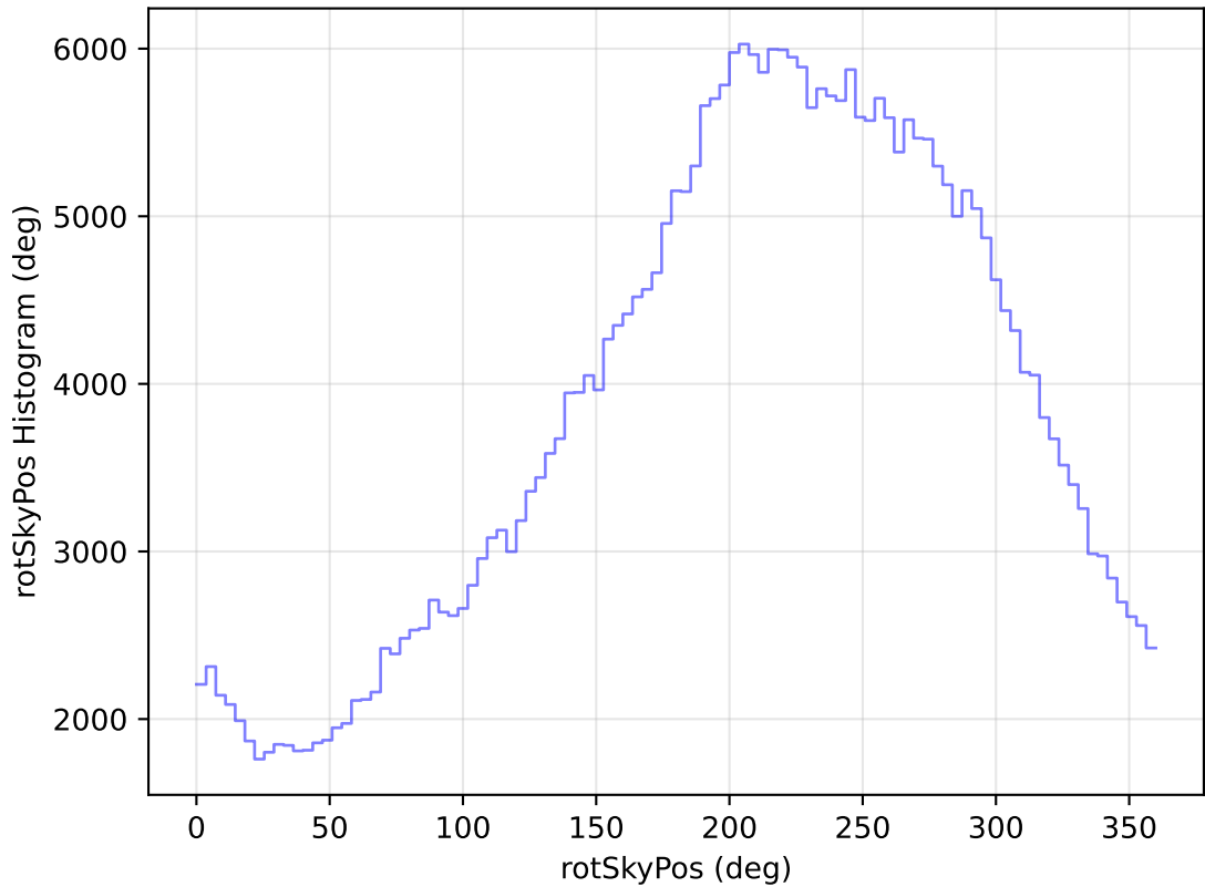
internal_u_expt45_nscale1.0v3.4_10yrs All sky y band: rotSkyPos Histogram
