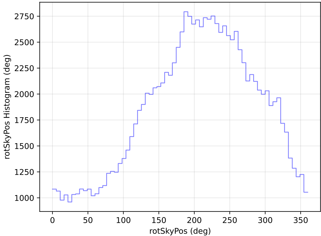
internal_u_expt45_nscale1.0v3.4_10yrs All sky u band: rotSkyPos Histogram
