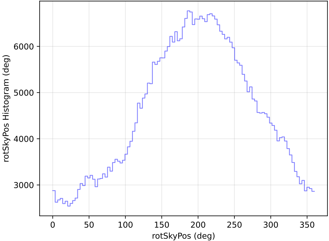
internal_u_expt45_nscale1.0v3.4_10yrs All sky r band: rotSkyPos Histogram
