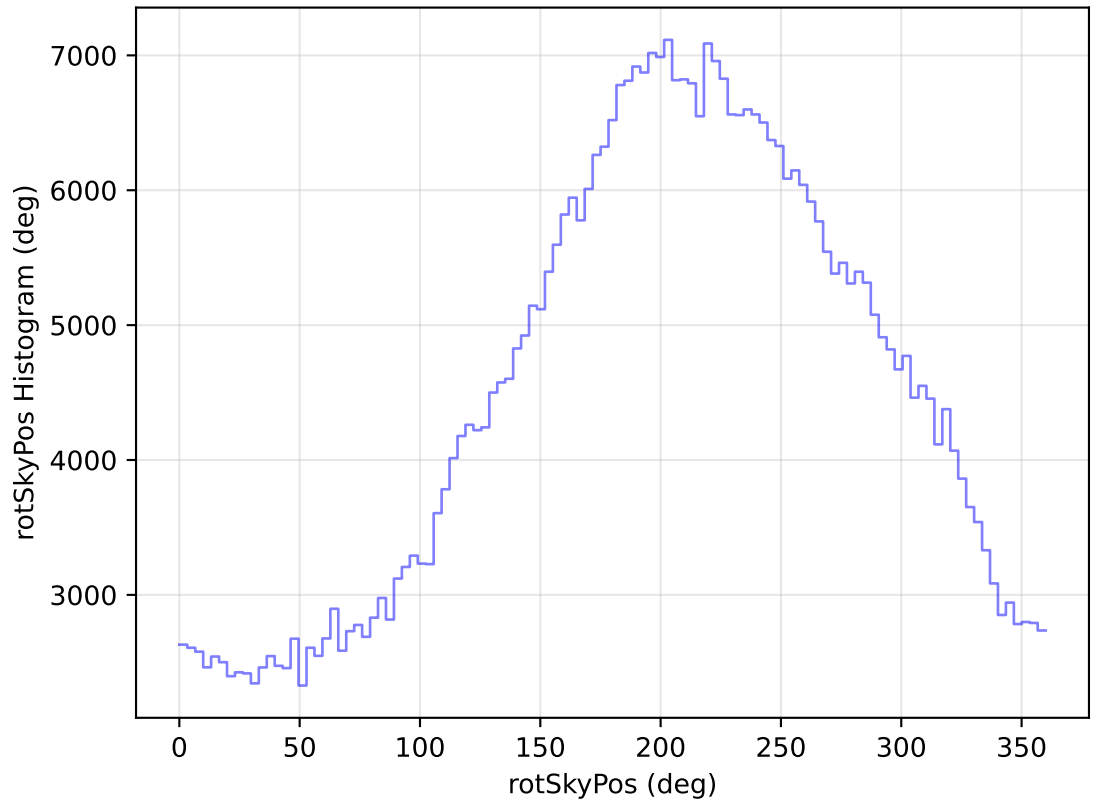
internal_u_expt45_nscale1.0v3.4_10yrs All sky i band: rotSkyPos Histogram
