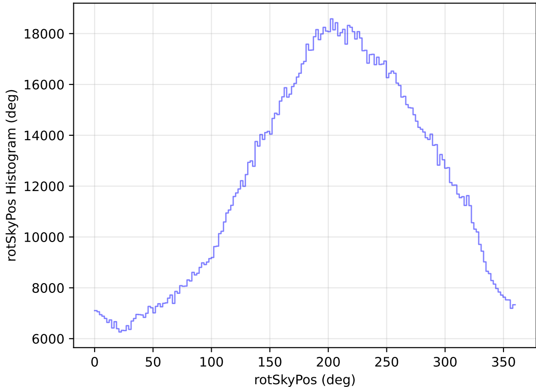
internal_u_expt45_nscale1.0v3.4_10yrs All sky all bands: rotSkyPos Histogram
