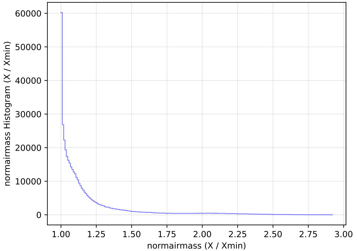
internal_u_expt45_nscale1.0v3.4_10yrs WFD z band: normairmass Histogram
