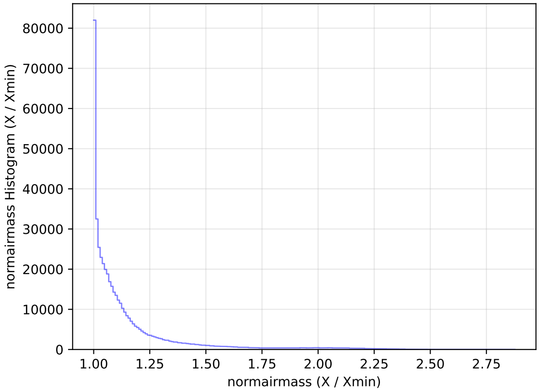
internal_u_expt45_nscale1.0v3.4_10yrs WFD r band: normairmass Histogram
