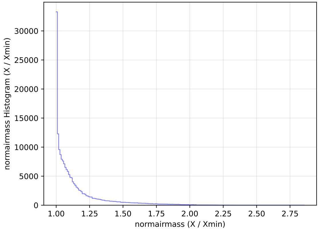
internal_u_expt45_nscale1.0v3.4_10yrs WFD g band: normairmass Histogram
