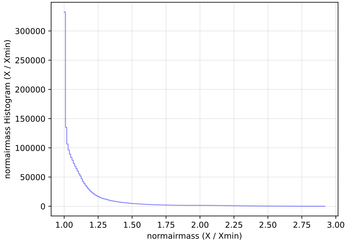
internal_u_expt45_nscale1.0v3.4_10yrs WFD all bands: normairmass Histogram
