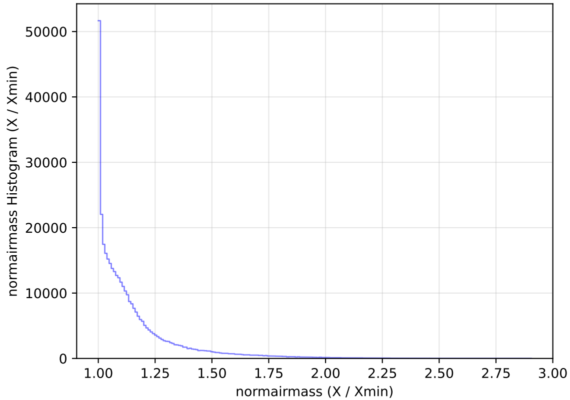
internal_u_expt45_nscale1.0v3.4_10yrs All sky y band: normairmass Histogram
